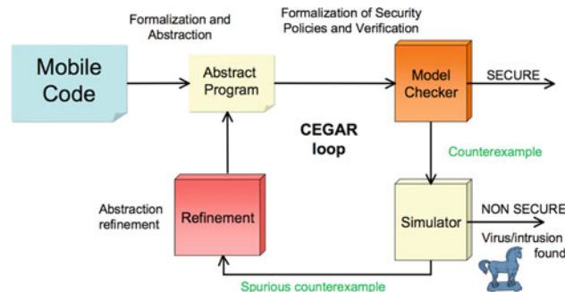
Fig. 5. The CEGAR loop
