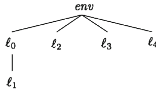
Fig. 2. The location net of Example 3
