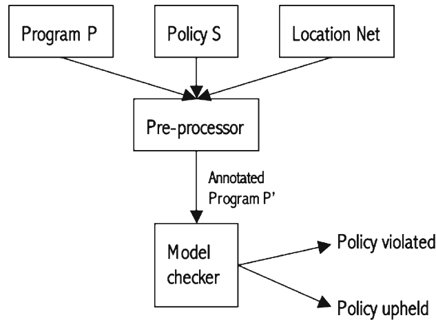
Fig. 4. The experimental framework
