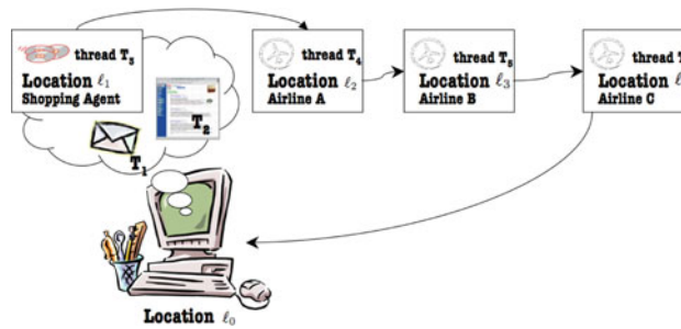
Fig. 1. A shopping agent. Here, \ell_0 to \ell_4 are locations representing sites, and T_1 to T_6 threads
